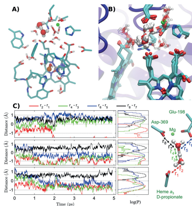
Figure 2. Structure and dynamics of the protonated water cluster above the D-propionate of heme a_3 . A) Optimized protonated water cluster in the P_M state from a DFT model with 340 atoms. B) Snapshots from QM/MM dynamics of the protonated water cluster from a 5 ps trajectory with about 130 QM atoms and about 88 700 MM atoms. C) QM/MM dynamics and probability distributions of the central oxygen-hydrogen distance differences, shown in inset to the right. A value near 0 Å, indicates a proton shared between two oxygens, while values > +1.0 / < -1.0 Å indicate regular hydrogen bonds. The three panels show the dynamics in the a^{\text{ox}}/P_M (top), a^{\text{red}}/P_M (middle), a_{\text{ox}}/F (bottom) states.
